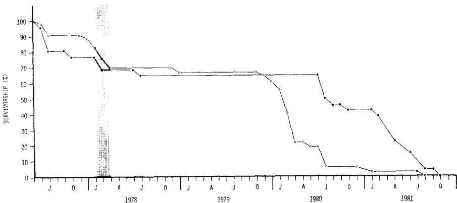
Fig. 1.—Survivorship (%) as a function of time in two litters of Centruroides gracilis born and raised in the laboratory. Hatched region (February-April 1978) represents the final molt (to sexual maturity). Solid circles = litter I ( n = 26 ); open circles = litter II ( n = 46 ).
