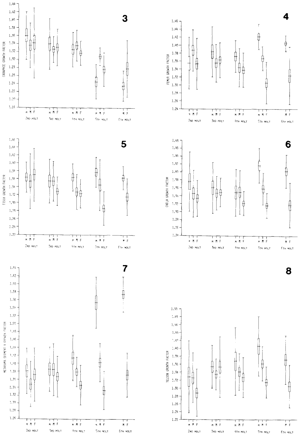
Figs. 3-8.—Growth factors (GF = “Dyar’s constant”) per molt for small males (m), large males (M), and females (F) from two litters of Centruroides gracilis born and raised in the laboratory. Small males are sexually mature after the fifth molt (i. e., at the sixth instar) and cease to molt thereafter. Shown are the mean, \pm one standard error of the mean (box), and \pm one standard deviation. 3, Carapace length GF; 4, Pedipalp femur length GF; 5, Tibia length GF; 6, Chela length GF; 7, Metasomal segment V length GF; 8, Telson length GF.
