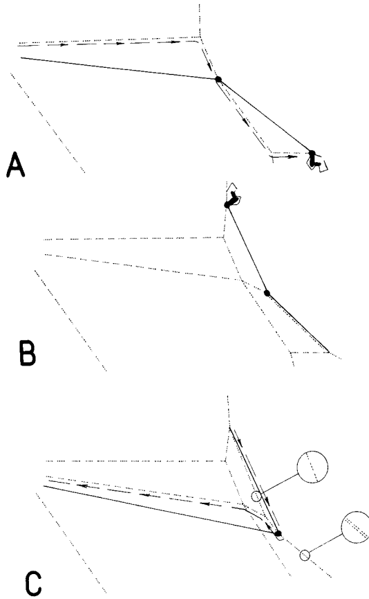
Figure 25.—Sequence of events in complex N. clavipes frame construction behavior (conventions as in Figs. 3 and 4).
