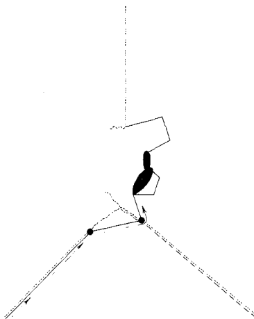
Figure 14.—Details of last attachment in frame construction sequences of L. mariana (e.g., D in Figs. 12, 13). As the spider breaks the radius (vertical line) it attaches to the frame on both sides of the original radius-frame attachment, thus allowing a short segment of the frame to go slack (conventions as in Fig. 3).
