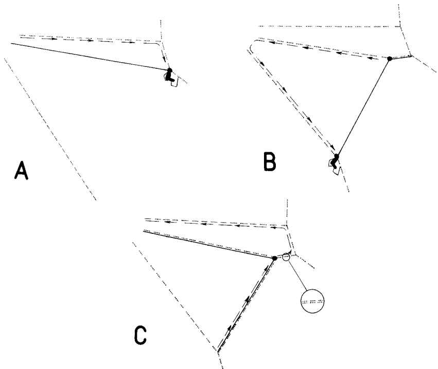
Figure 20.—Sequence of events in N. clavipes frame construction similar to that in Fig. 17 except the spider attached the second radius right at the point on the frame where the first was attached (C) (conventions as in Figs. 3 and 4).
