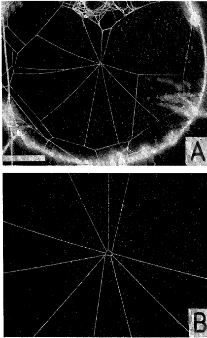
Figure 2. Web of P. vicina : A, just after protohub replacement (one radius was laid after the protohub was removed); B, closeup of hub of this web. The loose silk is gone, and the radii are connected by an approximately circular line that was laid as the loose silk was removed.
