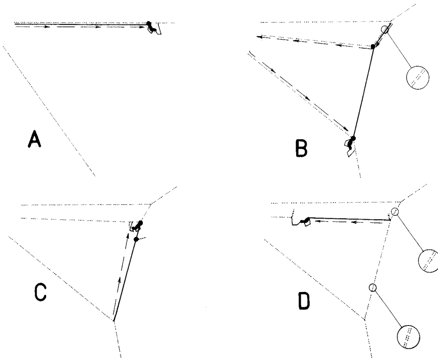
Figure 8.—Sequence of events in P. vicina frame construction Type E (conventions as in Figs. 3 and 4).
