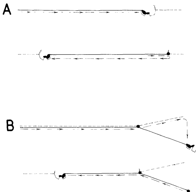
Figure 3.—Two types of partial replacement of radii: Dashed lines with arrows show the route taken by the spider's feet, dotted lines are lines already present, intact lines are those newly laid in each drawing, and large dots mark new attachments. A, the spider breaks and reels up the exit radius while moving away from the hub (above), then turns and replaces the newly laid dragline by breaking and reeling on the way back (below); B, the spider leaves the exit line intact as it leaves the hub, attaches its dragline to the exit on the way out and then moves onward and sideways (above). After making an attachment to the substrate or other lines, it returns, replacing the newly laid dragline and its attachments to other lines with another dragline and attachments (below).
