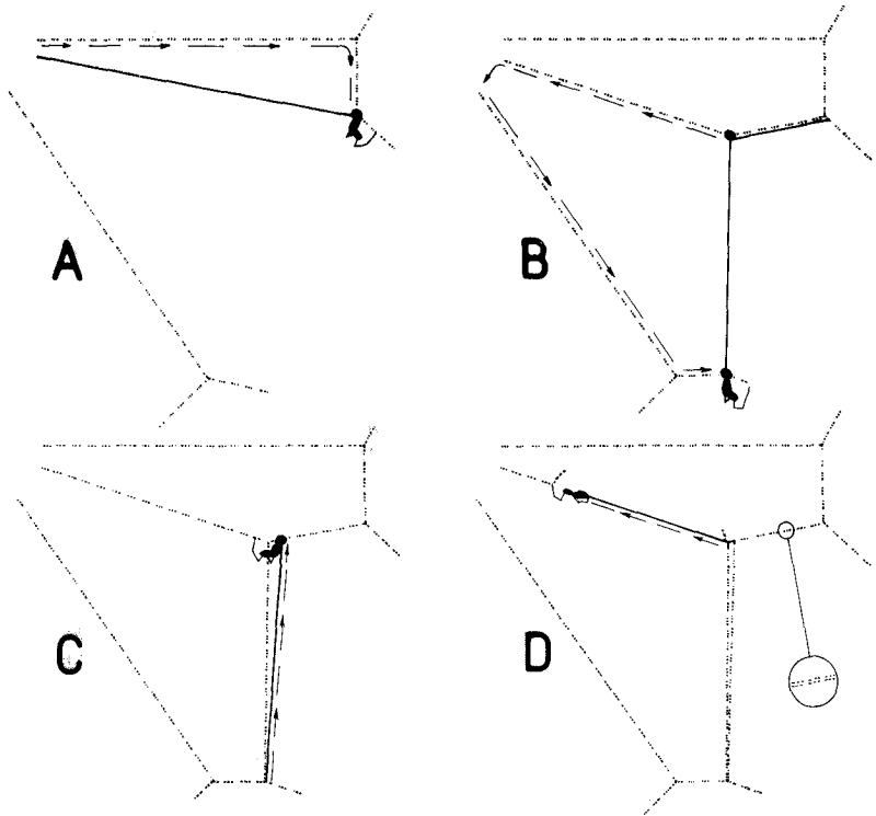
Figure 10.—Sequence of events in L. mariana frame construction Type A (conventions as in Figs. 3 and 4).
