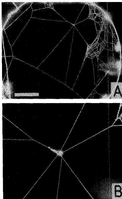
Figure 1.—Web of Philoponella vicina : A, nearly complete proto-web; B, closeup of the proto-hub, showing large accumulation of loose silk and lack of hub lines connecting radii.
