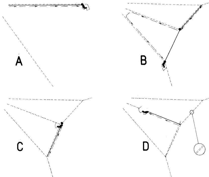
Figure 12.—Sequence of events in L. mariana frame construction Type C (conventions as in Figs. 3 and 4).
