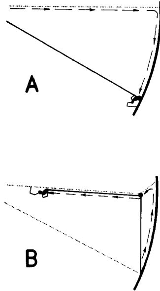
Figure 26.—A simple, feasible frame construction sequence which is apparently never used by orb weavers, in which the spider fails to return to the hub along a newly laid radial line (B).
