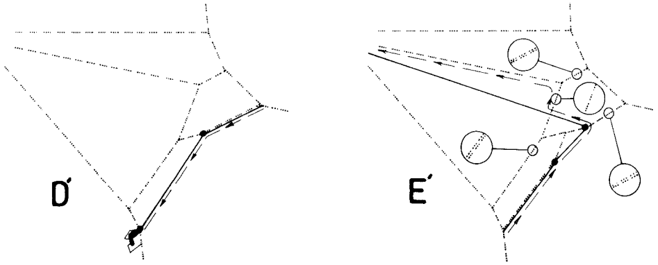
Figure 19.—Sequence of late events in N. clavipes frame construction. Behavior was similar to that in Fig. 18 (stages A-C were identical) except the spider made a trip across the entire sector (D') before crossing to lay the second radius and return to the hub (E') (conventions as in Figs. 3 and 4).
