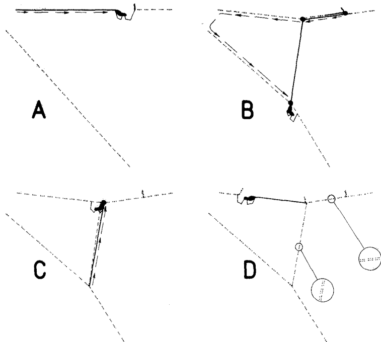
Figure 11.—Sequence of events in L. mariana frame construction Type B (conventions as in Figs. 3 and 4).
