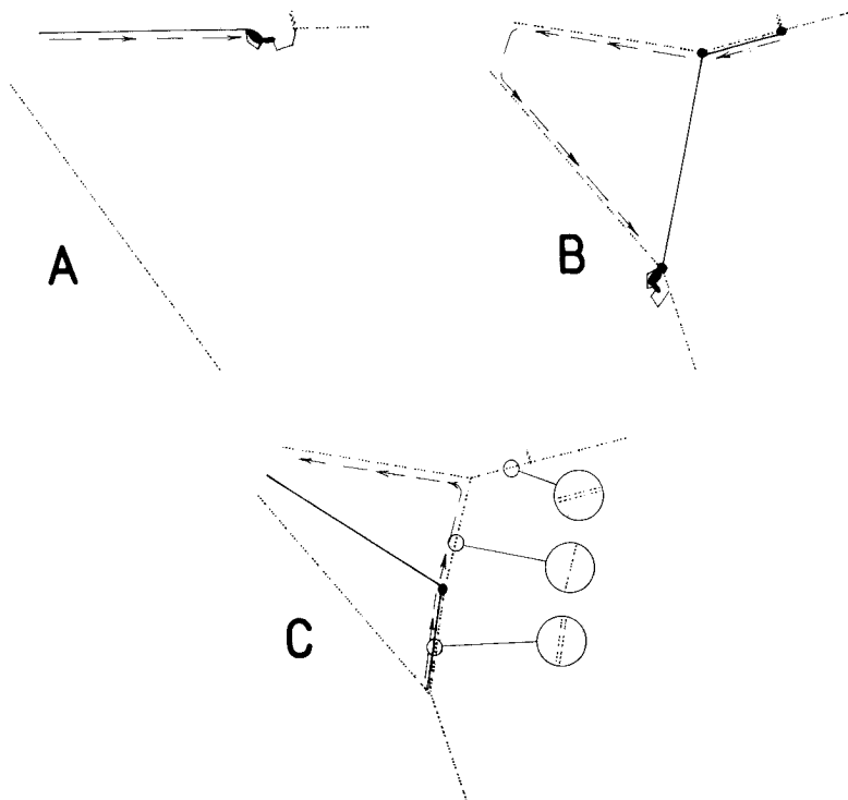
Figure 23.—Sequence of events in N. clavipes frame construction similar to that in Fig. 17 except the previous radius on which the spider moved away from the hub was broken and replaced (A) (conventions as in Figs. 3 and 4).
