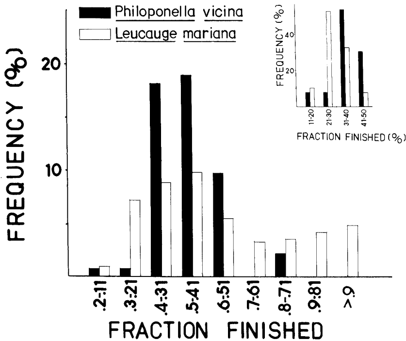
Figure 15.—Relative numbers of partial replacements at different stages of orb construction by P. vicina ( N = 72 replacements in 17 webs) and L. mariana ( N = 154 replacements in 40 orbs) (state of construction indicated by fraction of final number of radii already built). Since some observations began after the first radii had been laid, replacements made in the very earliest stages ( <0.20 ) are under-represented (inset shows the percentage of the final number of radii already present when observations began).
