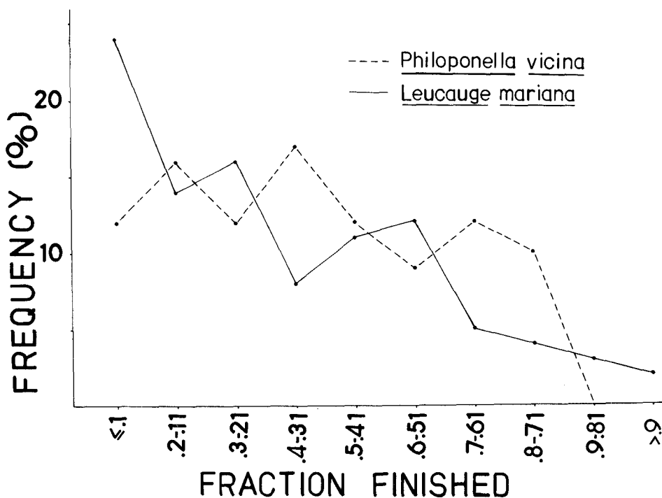
Figure 9.—Relative numbers of frame lines built at different stages of orb construction by P. vicina (dotted line) ( N = 58 frames in 17 orbs) and L. mariana (solid line) ( N = 92 frames in 18 webs) (stage of construction indicated by fraction of final number of radii already present). Since some observations began after the first few radii had been laid (inset in Fig. 15), the frames laid in the very earliest stages ( < 0.20 ) are under-represented.
