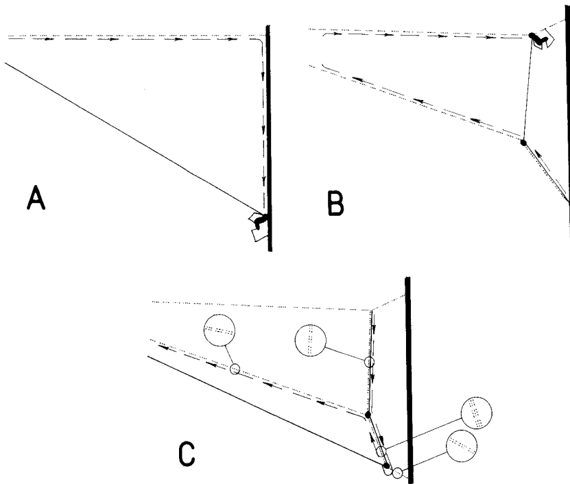
Figure 21.—Sequence of events in N. clavipes frame construction similar to that in Fig. 17 except the spider moved along the new frame past the site of the first new radius before attaching the second new radius (C) (conventions as in Figs. 3 and 4).
