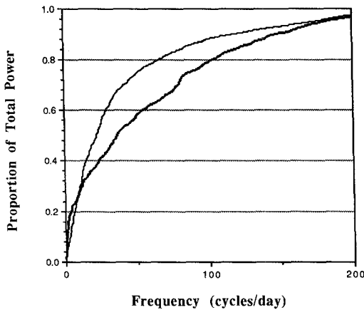
Figure 21.—Cumulative explained variance in the spectral analyses of the activity records of two F. pyramitela . The heavy line corresponds to the analysis of the data shown in Fig. 2 and the light line corresponds to the analysis of the data shown in Fig. 7. The most rapid rise in explained variance occurs very near the origin, indicating that high frequencies ( > 75 cycles/day) are of minor importance (see text).
