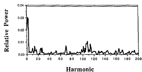
Figures 30–34.—Patterns in the durations of intervals between bouts of activity by A. trigonum in constant darkness (DD). See the legend to Figs. 23–29 for details of the layout. In none of the analyses was there significant power at harmonics above DC, an indication that the sequences of durations were not different from random.
