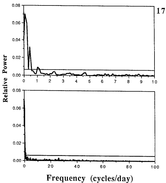
Figures 16–20.—Activity of A. trigonum under conditions of constant darkness (DD). See the legend for Figs. 2–8 for an explanation of the layout.
