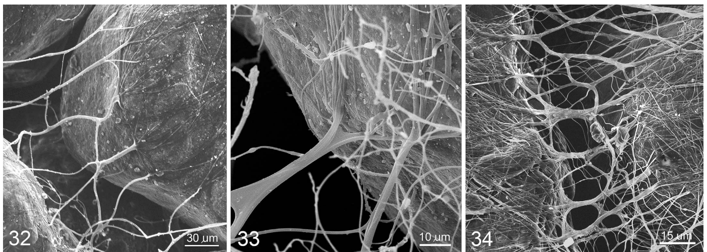
Figures 32–34.—Silk fibers connecting neighboring sand grains arise from very fine threads on the surface of a sand grain, which then coalesce into thicker fiber bundles. 32. Tube wall of C. rechenbergi . 33. Same as in Fig. 25, but in higher magnification (Photo: A. C. Joel). 34. Tube wall of A. senex .
