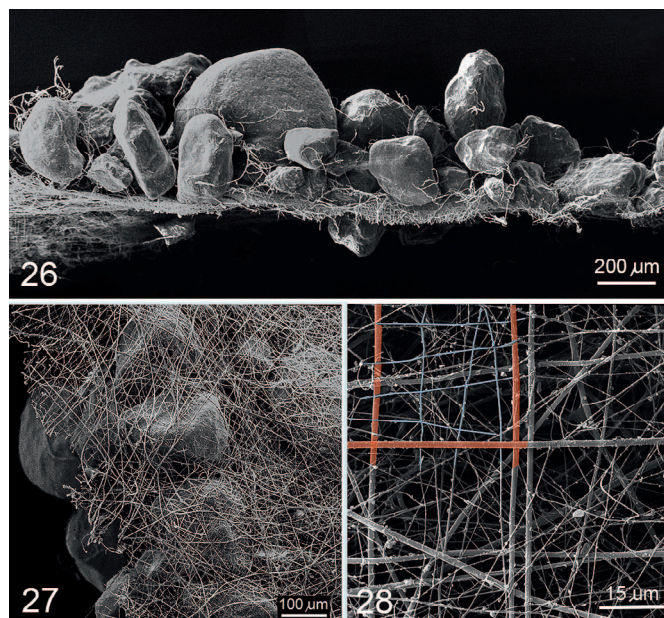
Figures 26–28.—Structure of the burrow wall in C. rechenbergi . 26. Cross section of the lid in lateral view. Note that only 1–2 layers of sand grains are attached to the thin silk mat. 27. Inside of the burrow wall showing fine silk threads crossing several sand grains. 28. A high magnification of the silk lining reveals a mesh of thick fibers (marked in red) overlying a fine mesh of thin fibers (in blue).
