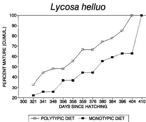
Figure 2.—Cumulative (percent) maturation curves for laboratory populations of Lycosa helluo from Florida raised on different diets. Open squares/solid line—polytypic diet; filled squares/dashed line—monotypic diet.
