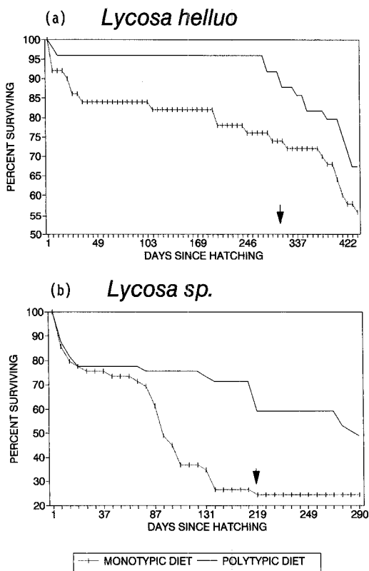
Figure 1.—Survivorship (in days) of laboratory populations of lycosids raised on different diets. Solid line—polytypic diet; dashed line—monotypic diet. Arrows indicate approximate earliest onset of sexual maturity. a : Lycosa helluo from Florida; b : Lycosa sp. from Kentucky.
